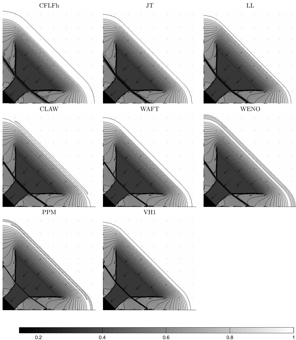
FIG. 4.10. Results for the implosion problem at early stage by all eight schemes. Color pressure map is overlaid by 36 density contours (0.125 to 1 step 0.025) and velocity arrows. The computations were done on the square (x, y) \in (0, 0.3) \times (0, 0.3) with 400 \times 400 grid to time T = 0.045 and is presented on the square (0, 0.22) \times (0, 0.22) .
