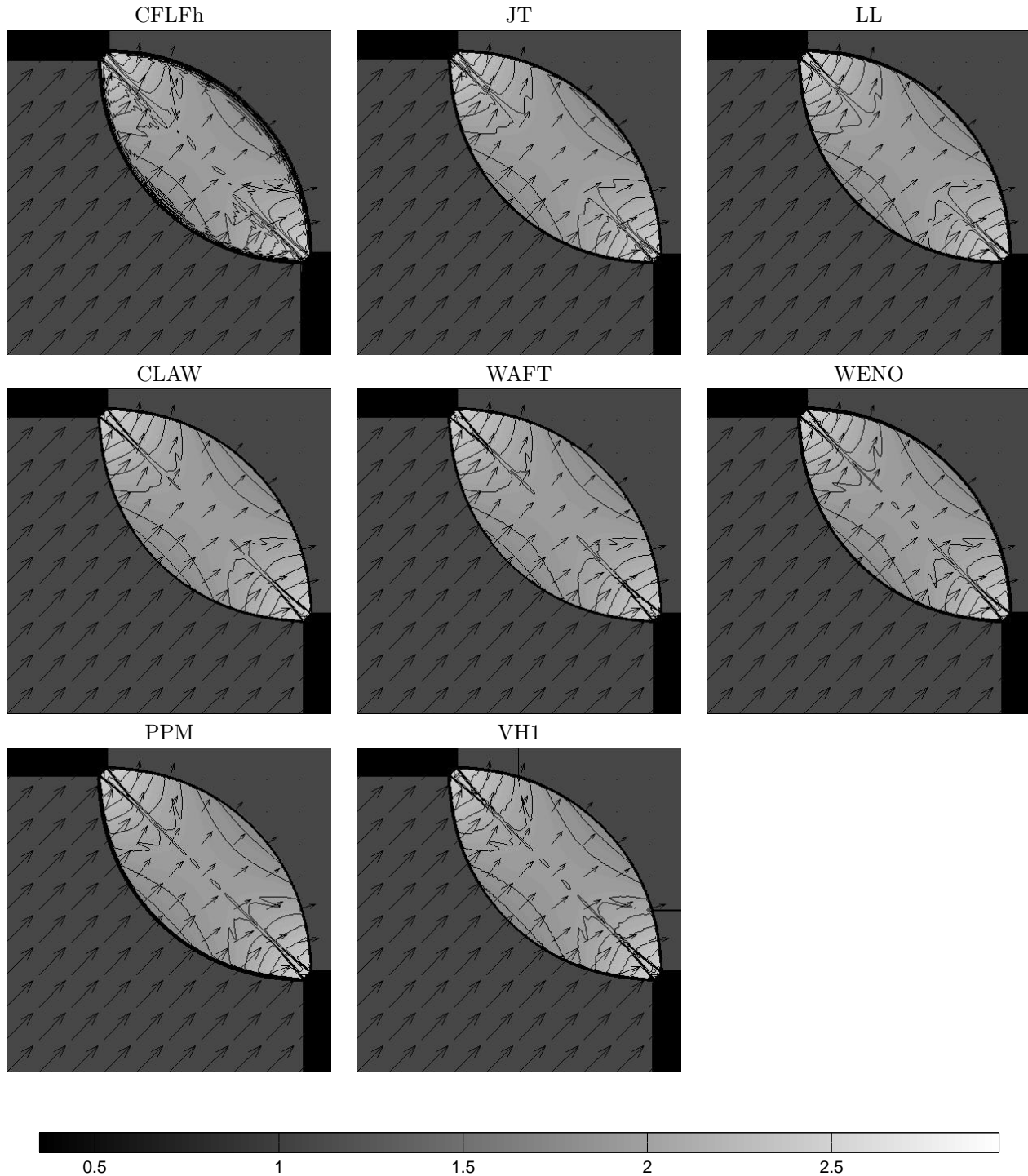
FIG. 4.2. Results for the 2D Riemann problem case 4 by all eight schemes. Pressure is displayed by color, density by 29 contours (0.52 to 1.92 step 0.05) and velocity by arrows. For all cases the computations were done and are presented on the square (x, y) \in (0, 1) \times (0, 1) .
