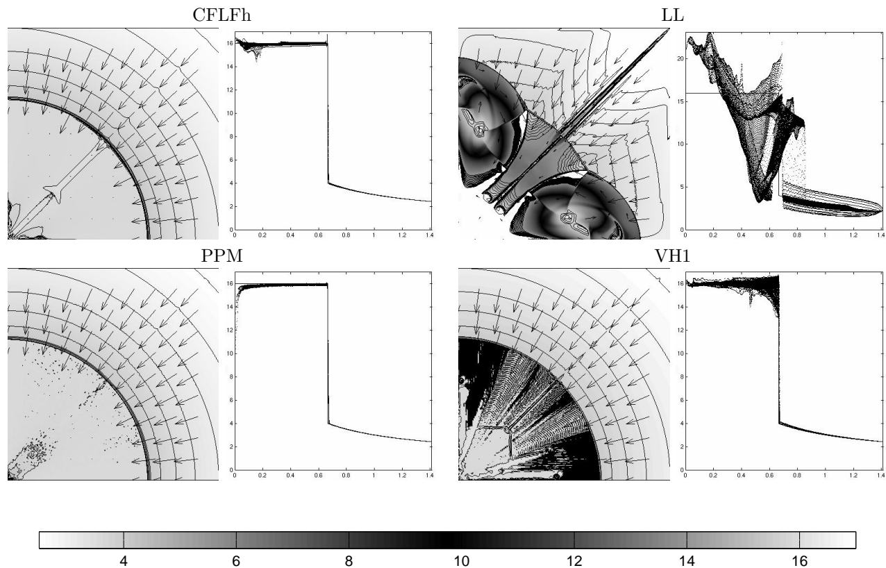
FIG. 4.7. Results for the Noh problem by the CFLFh, LL, PPM and VH1 schemes. JT, CLAW, WAFT and WENO have failed for this problem. Density color map is overlaid by 23 density contours ( 2.5 to 4 step 0.25 and 14 to 17 step 0.2) and velocity arrows on the left. Scatter plot of density versus radius is on the right. The computations were done on the square (x, y) \in (0, 1) \times (0, 1) with 400 \times 400 grid to time T = 2 .
