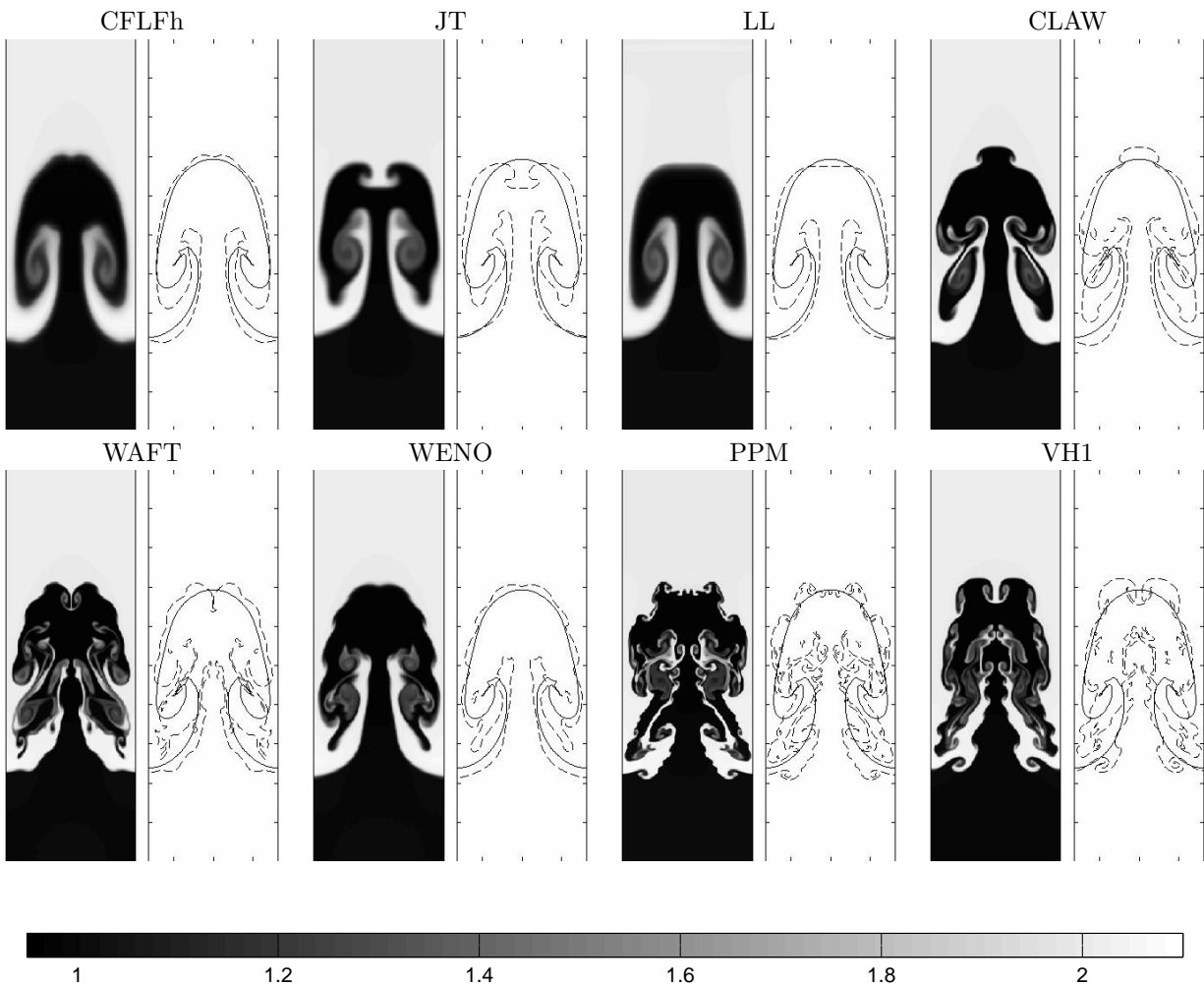
FIG. 4.8. Results for the Rayleigh-Taylor problem by all eight schemes. Density color map and front contour. The solid line in the contour plots is the result of a front tracking code. The computations were done on the rectangle (x, y) \in (0, 1/6) \times (0, 1) with 100 \times 400 grid to time T = 8.5 .
