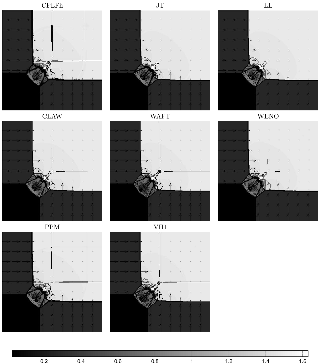
FIG. 4.1. Results for the 2D Riemann problem case 3 by all eight schemes. Pressure is displayed by color, density by 32 contours (0.16 to 1.71 step 0.05) and velocity by arrows. For all cases the computations were done and are presented on the square (x, y) \in (0, 1) \times (0, 1) .
