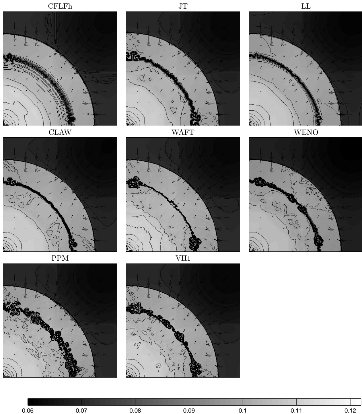
FIG. 4.12. Results for the explosion problem by all eight schemes. Color pressure map is overlaid by 27 density contours (0.08 to 0.21 step 0.005) and velocity arrows. Computations were done on the square (x, y) \in (0, 1.5) \times (0, 1.5) with 400 \times 400 grid till time T = 3.2 .
