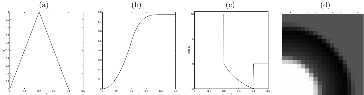
FIG. 4.14. Exact solution of the Gresho problem: dependence of angular velocity (a), pressure (b) and vorticity (c) on radius; initial vorticity on 40 \times 40 grid (d).
