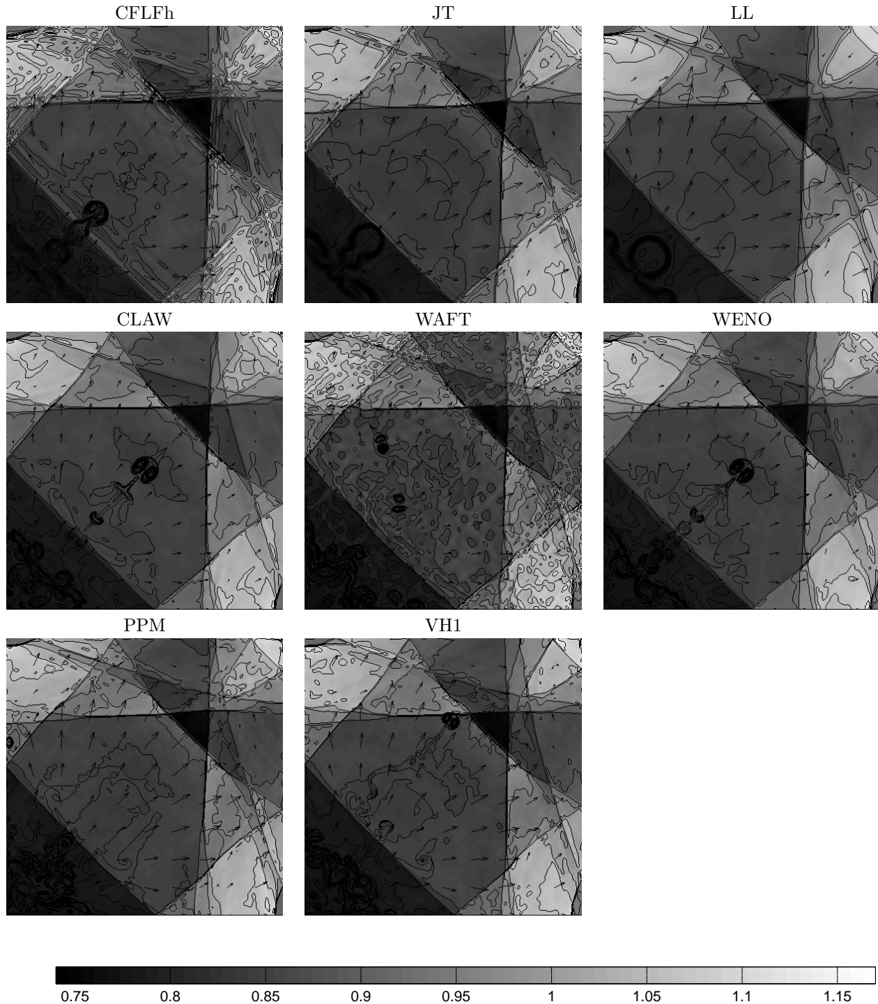
FIG. 4.11. Results for the implosion problem at late stage by all eight schemes. Color pressure map is overlaid by 31 density contours (0.35 to 1.1 step 0.025) and velocity arrows. The computations were done on the square (x,y) \in (0,0.3) \times (0,0.3) with 400 \times 400 grid to time T = 2.5 .
