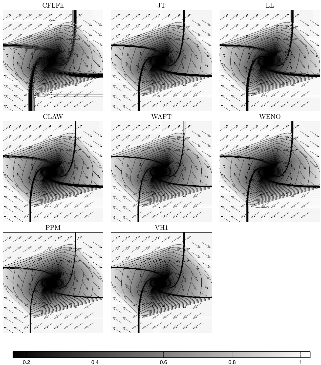
FIG. 4.3. Results for the 2D Riemann problem case 6 by all eight schemes. Pressure is displayed by color, density by 29 contours (0.25 to 3.05 step 0.1) and velocity by arrows. For all cases the computations were done and are presented on the square (x, y) \in (0, 1) \times (0, 1) .
